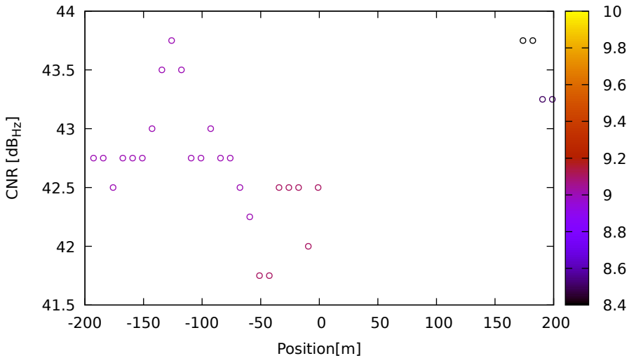
CNR vs position for E15 (E5a) on LeicaGS18 - DOY 262 jam. 3
