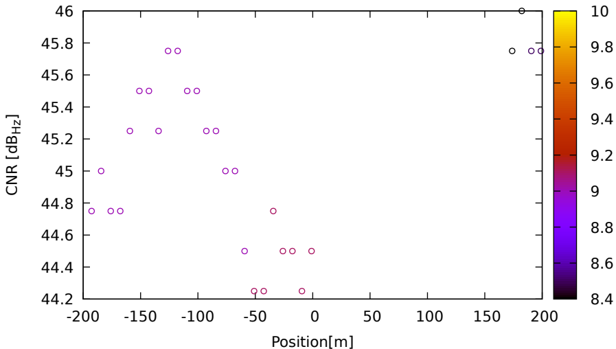
CNR vs position for E15 (E8) on LeicaGS18 - DOY 262 jam. 3
