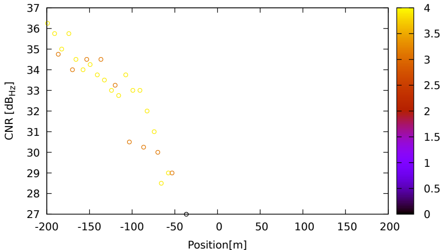
CNR vs position for E27 (E5b) on LeicaGS18 - DOY 262 jam. 1
