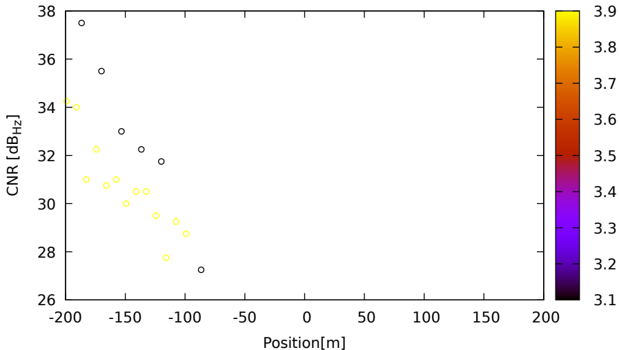
CNR vs position for E27 (E8) on LeicaGS18 - DOY 262 jam. 1
