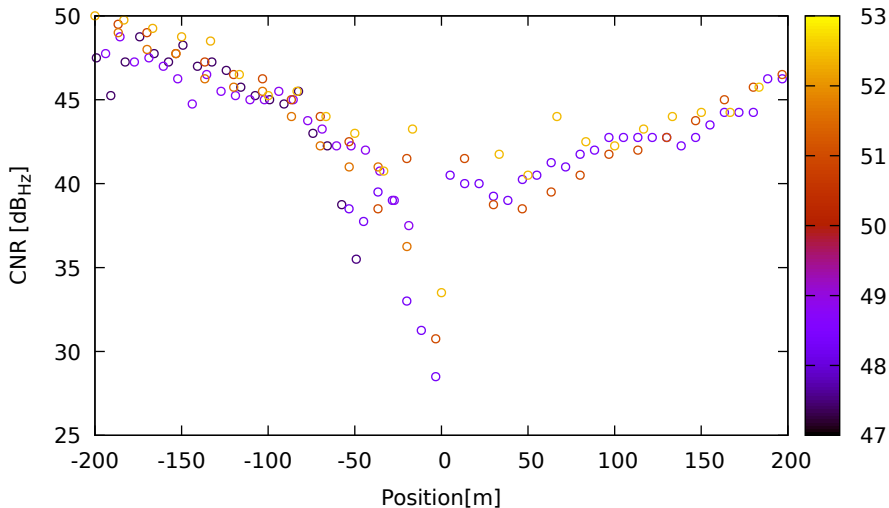
CNR vs position for E34 (E1) on LeicaGS18 - DOY 262 jam. 1
