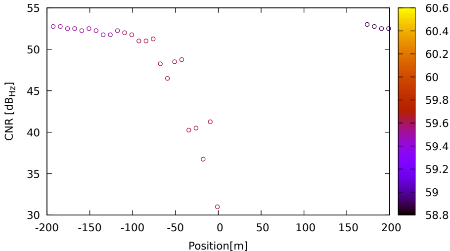
CNR vs position for E34 (E1) on LeicaGS18 - DOY 262 jam. 3
