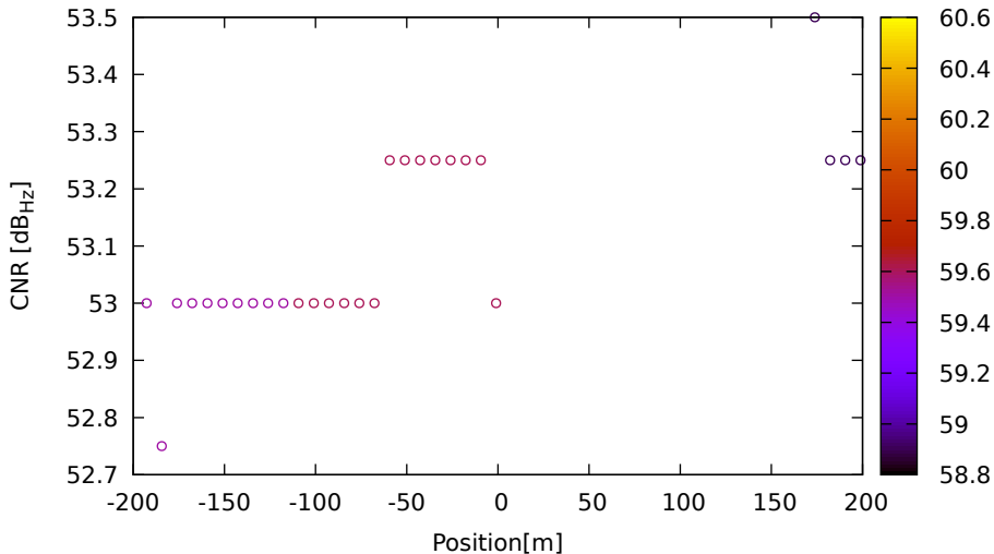
CNR vs position for E34 (E5a) on LeicaGS18 - DOY 262 jam. 3
