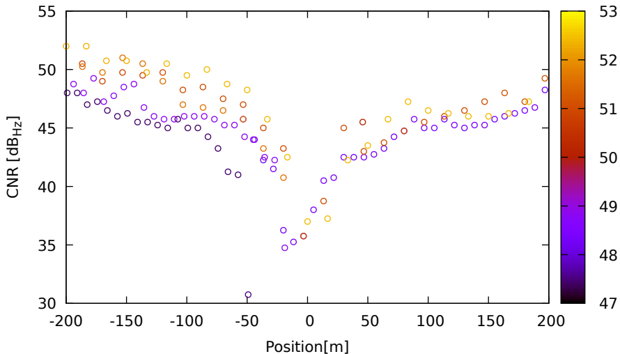
CNR vs position for E34 (E5b) on LeicaGS18 - DOY 262 jam. 1
