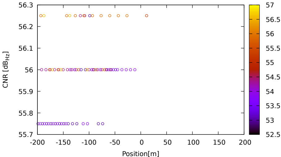
CNR vs position for E34 (E8) on LeicaGS18 - DOY 262 jam. 2
