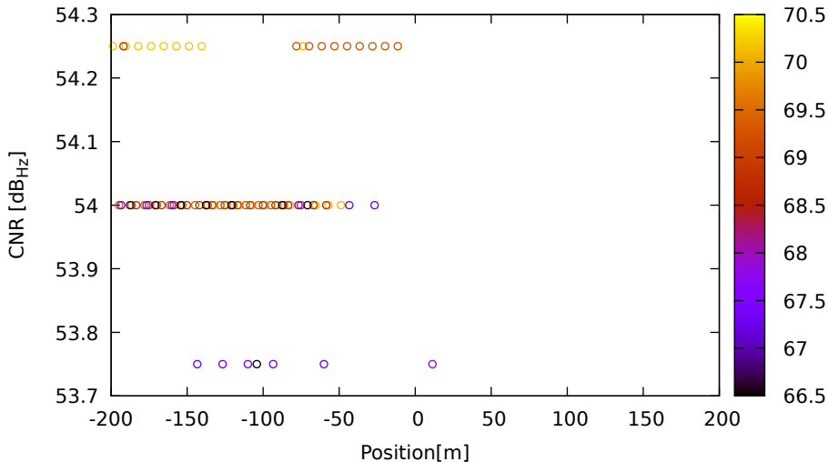
CNR vs position for E36 (E5a) on LeicaGS18 - DOY 262 jam. 2
