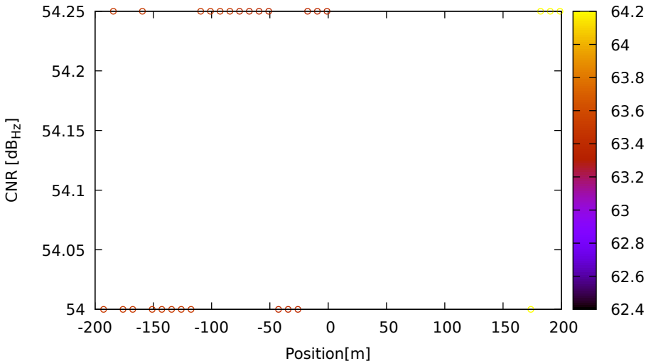
CNR vs position for E36 (E5b) on LeicaGS18 - DOY 262 jam. 3
