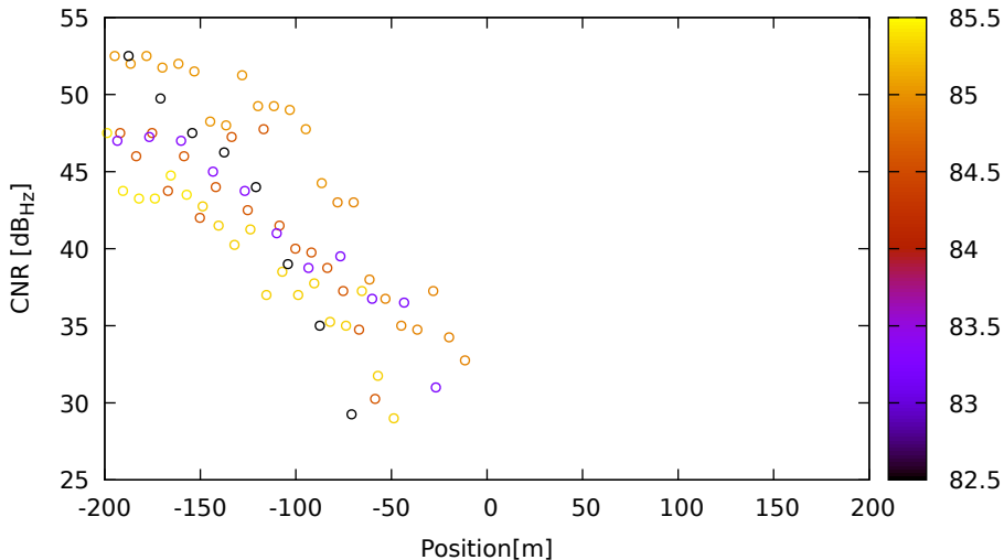
CNR vs position for G01 (L1) on LeicaGS18 - DOY 262 jam. 2
