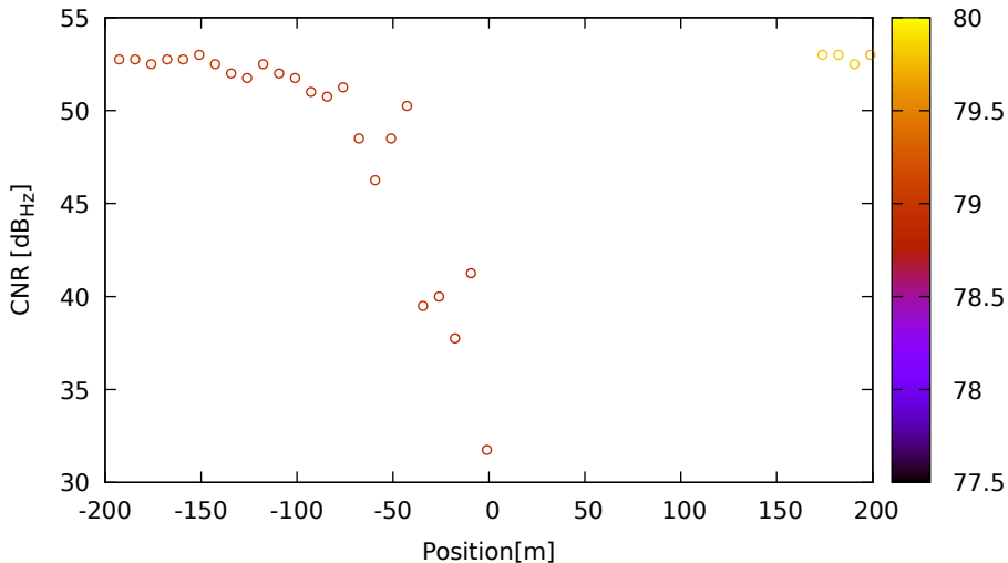
CNR vs position for G01 (L2) on LeicaGS18 - DOY 262 jam. 3
