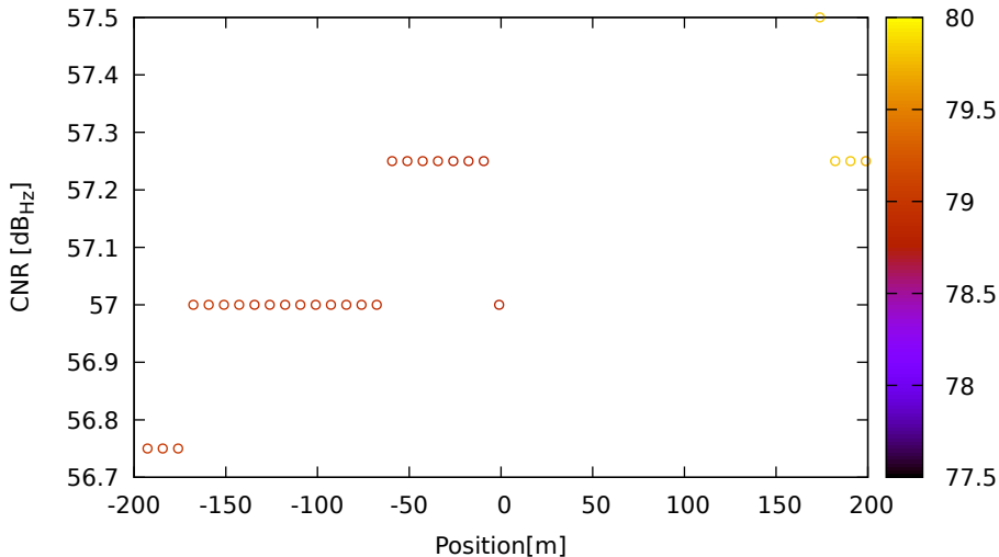
CNR vs position for G01 (L5) on LeicaGS18 - DOY 262 jam. 3
