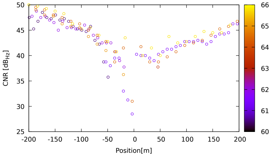
CNR vs position for G03 (L1) on LeicaGS18 - DOY 262 jam. 1
