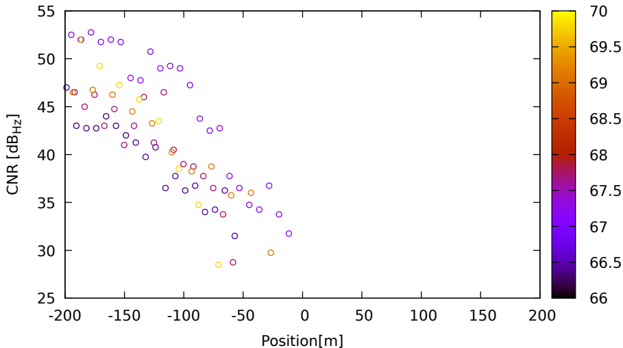
CNR vs position for G03 (L1) on LeicaGS18 - DOY 262 jam. 2
