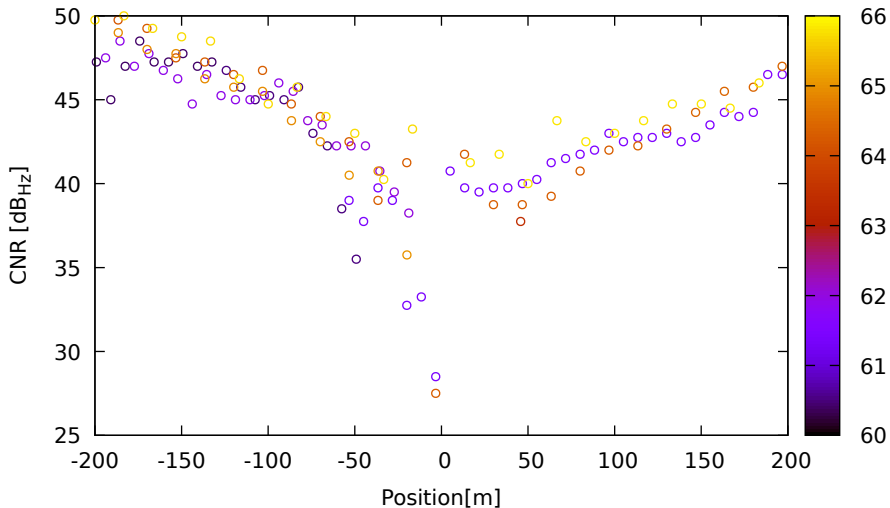
CNR vs position for G03 (L2) on LeicaGS18 - DOY 262 jam. 1
