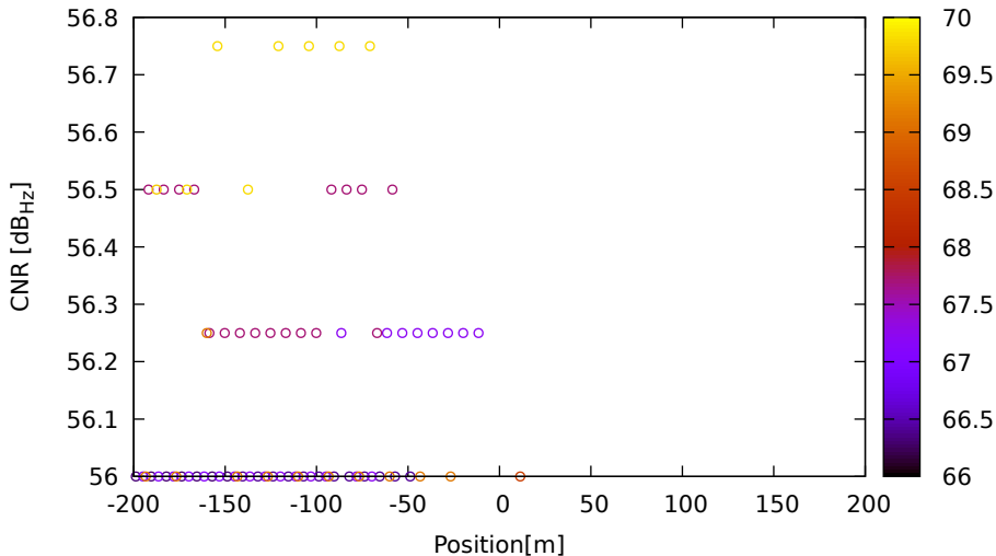
CNR vs position for G03 (L5) on LeicaGS18 - DOY 262 jam. 2
