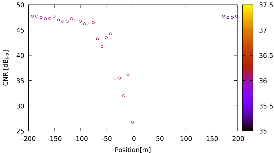
CNR vs position for G04 (L1) on LeicaGS18 - DOY 262 jam. 3
