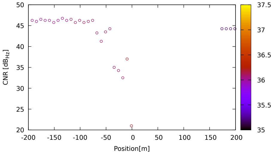
CNR vs position for G04 (L2) on LeicaGS18 - DOY 262 jam. 3
