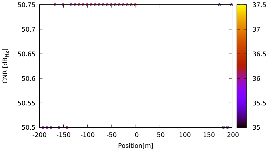
CNR vs position for G04 (L5) on LeicaGS18 - DOY 262 jam. 3
