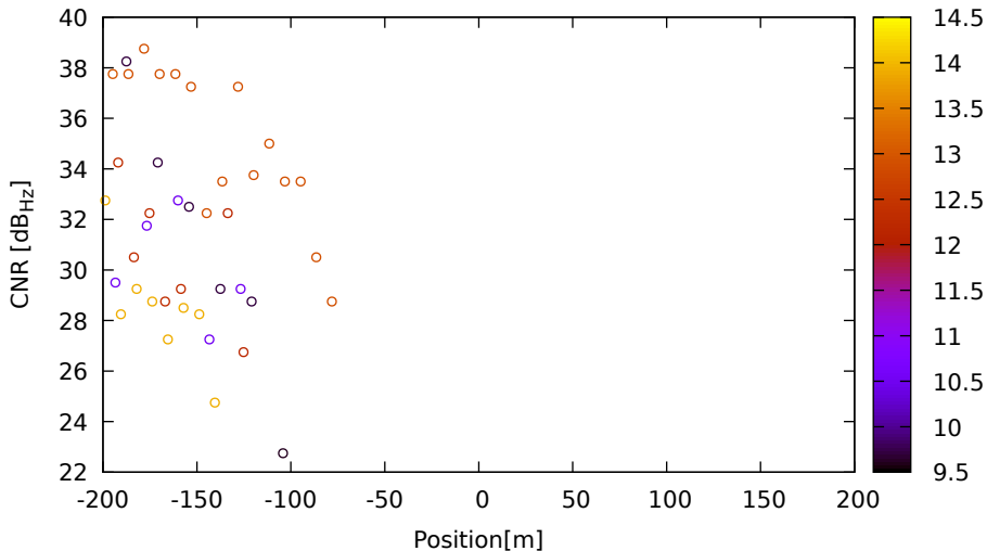
CNR vs position for G08 (L2) on LeicaGS18 - DOY 262 jam. 2
