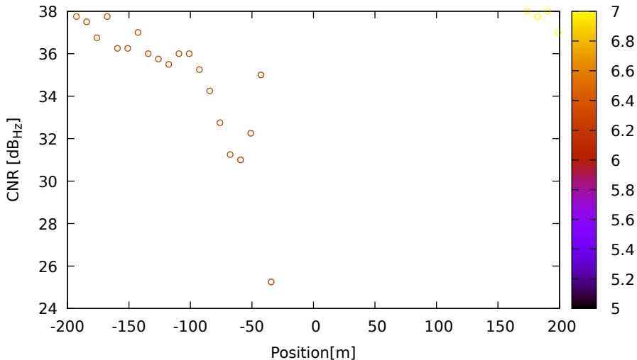
CNR vs position for G08 (L2) on LeicaGS18 - DOY 262 jam. 3
