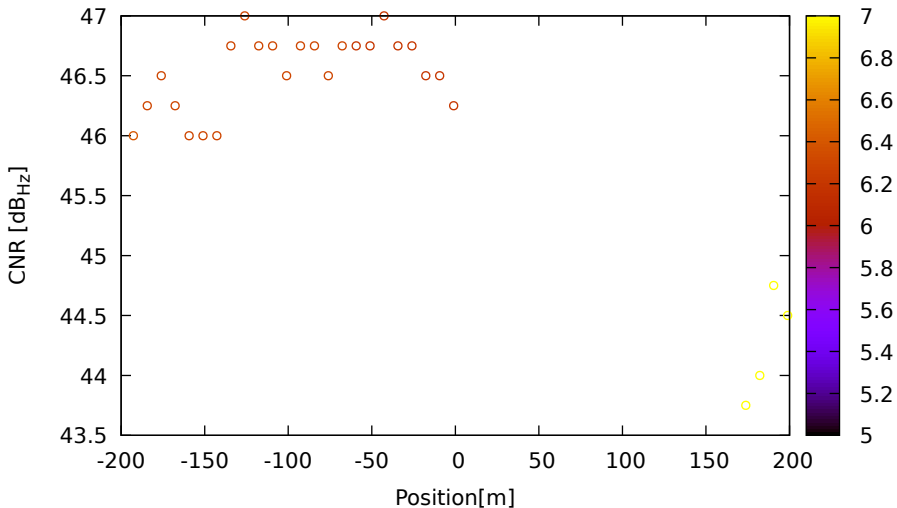
CNR vs position for G08 (L5) on LeicaGS18 - DOY 262 jam. 3
