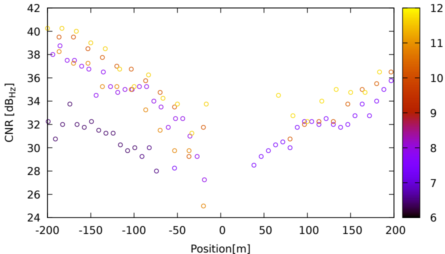
CNR vs position for G19 (L1) on LeicaGS18 - DOY 262 jam. 1
