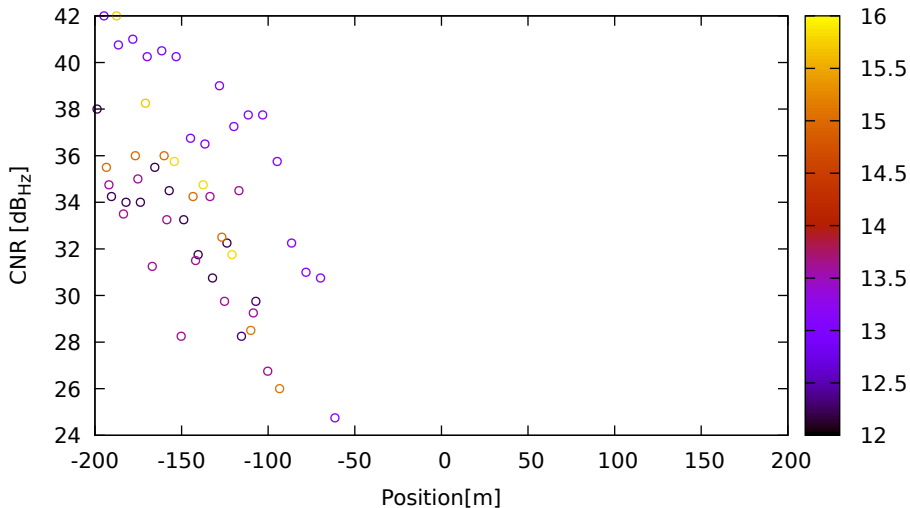
CNR vs position for G19 (L1) on LeicaGS18 - DOY 262 jam. 2
