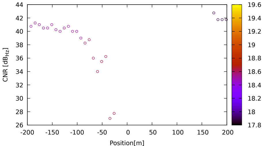
CNR vs position for G19 (L1) on LeicaGS18 - DOY 262 jam. 3
