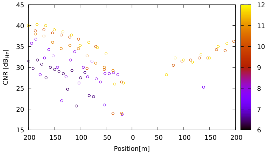
CNR vs position for G19 (L2) on LeicaGS18 - DOY 262 jam. 1
