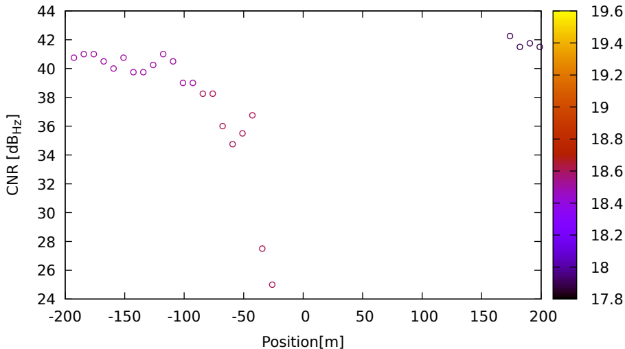
CNR vs position for G19 (L2) on LeicaGS18 - DOY 262 jam. 3
