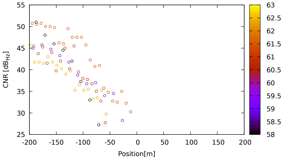
CNR vs position for G21 (L1) on LeicaGS18 - DOY 262 jam. 2
