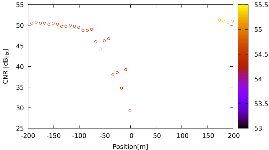
CNR vs position for G21 (L1) on LeicaGS18 - DOY 262 jam. 3
