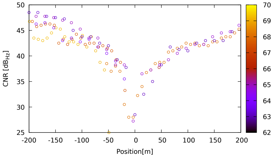
CNR vs position for G21 (L2) on LeicaGS18 - DOY 262 jam. 1
