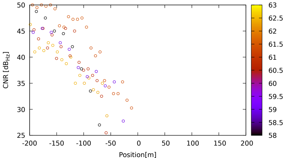
CNR vs position for G21 (L2) on LeicaGS18 - DOY 262 jam. 2
