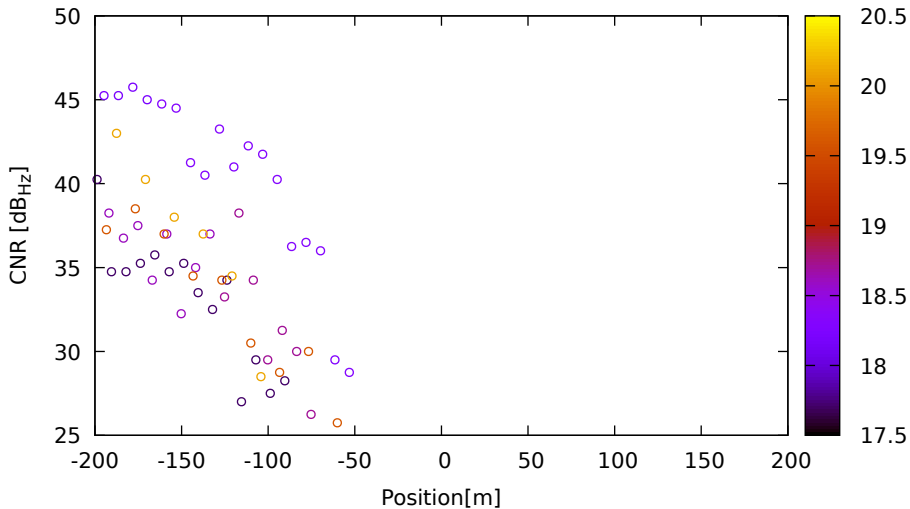
CNR vs position for G31 (L2) on LeicaGS18 - DOY 262 jam. 2
