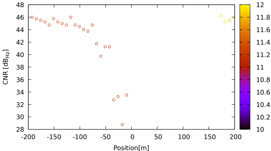
CNR vs position for G32 (L2) on LeicaGS18 - DOY 262 jam. 3
