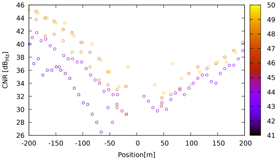
CNR vs position for R01 (G1) on LeicaGS18 - DOY 262 jam. 1
