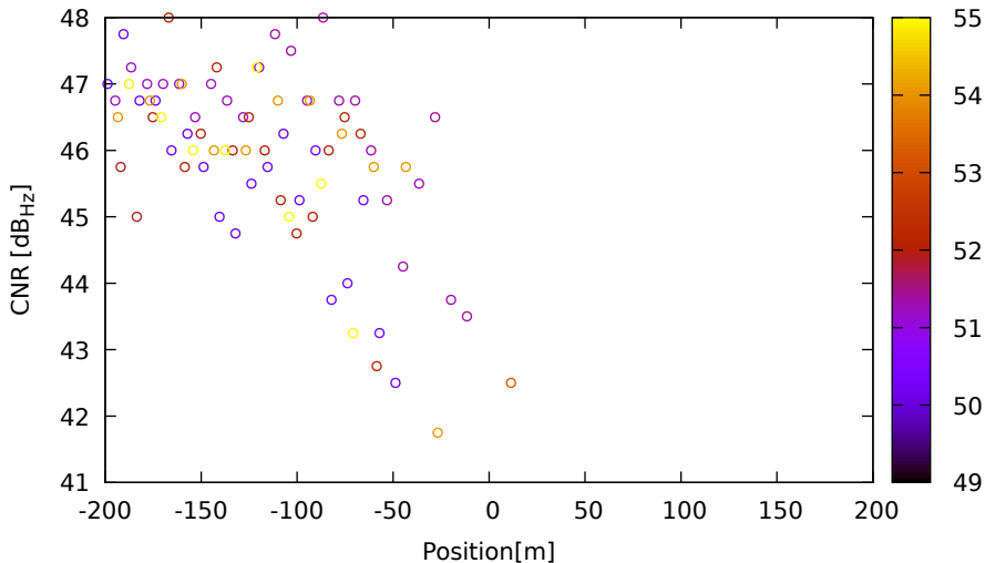
CNR vs position for R01 (G1) on LeicaGS18 - DOY 262 jam. 2
