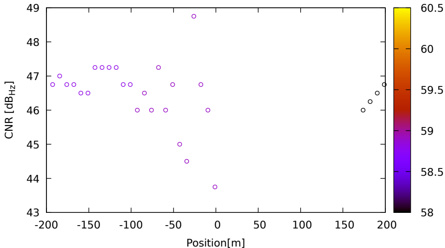
CNR vs position for R01 (G1) on LeicaGS18 - DOY 262 jam. 3
