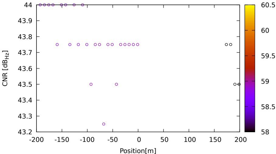
CNR vs position for R01 (G2) on LeicaGS18 - DOY 262 jam. 3
