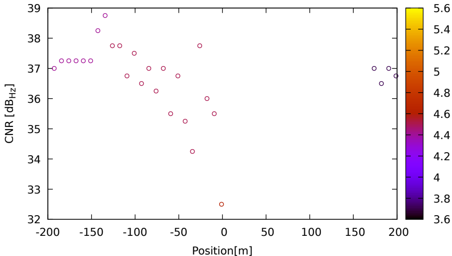
CNR vs position for R02 (G1) on LeicaGS18 - DOY 262 jam. 3
