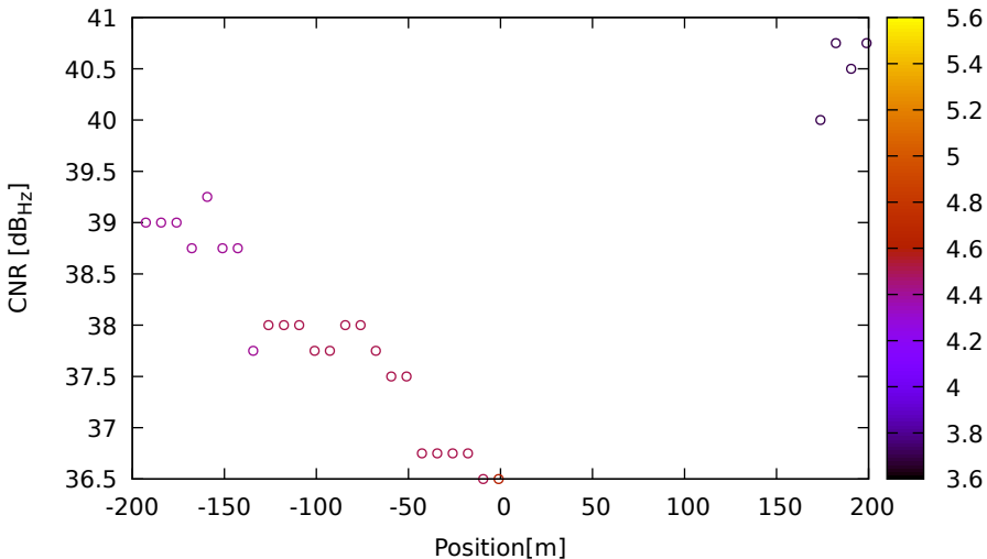
CNR vs position for R02 (G2) on LeicaGS18 - DOY 262 jam. 3
