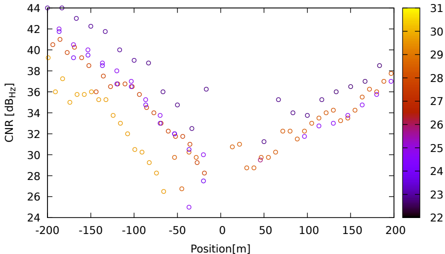
CNR vs position for R07 (G1) on LeicaGS18 - DOY 262 jam. 1
