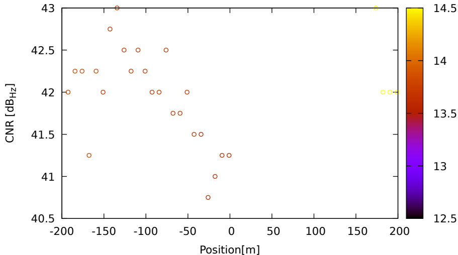
CNR vs position for R07 (G2) on LeicaGS18 - DOY 262 jam. 3
