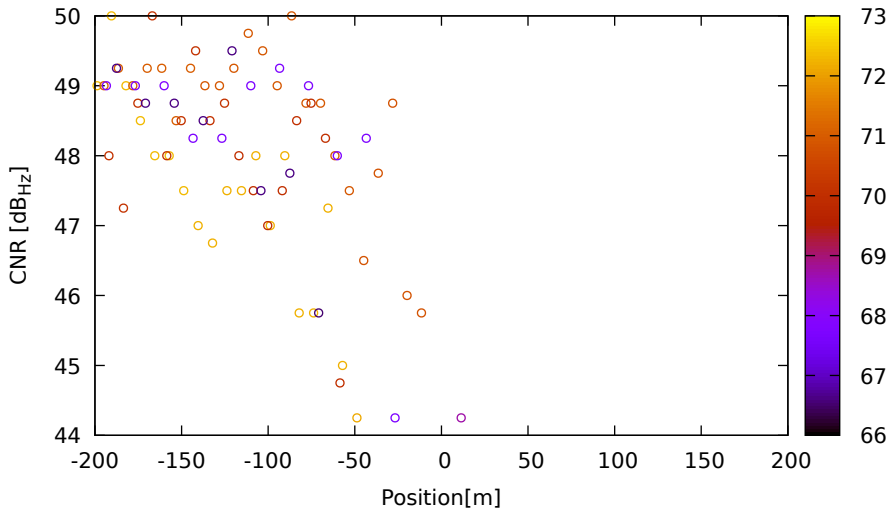
CNR vs position for R08 (G1) on LeicaGS18 - DOY 262 jam. 2
