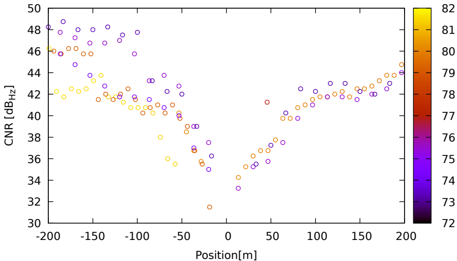
CNR vs position for R08 (G2) on LeicaGS18 - DOY 262 jam. 1
