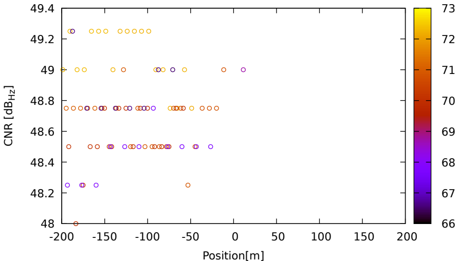
CNR vs position for R08 (G2) on LeicaGS18 - DOY 262 jam. 2
