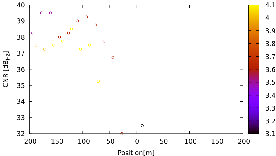
CNR vs position for R09 (G1) on LeicaGS18 - DOY 262 jam. 2
