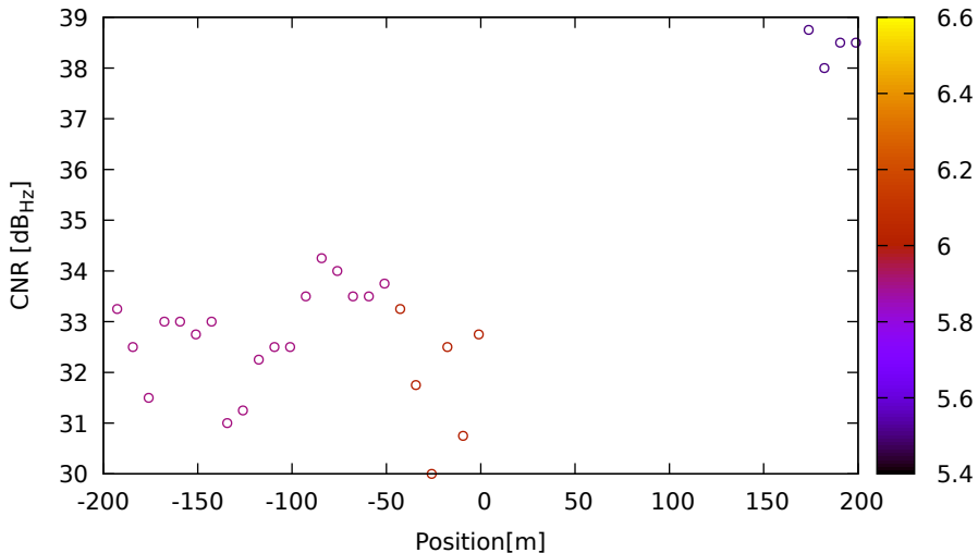
CNR vs position for R09 (G2) on LeicaGS18 - DOY 262 jam. 3
