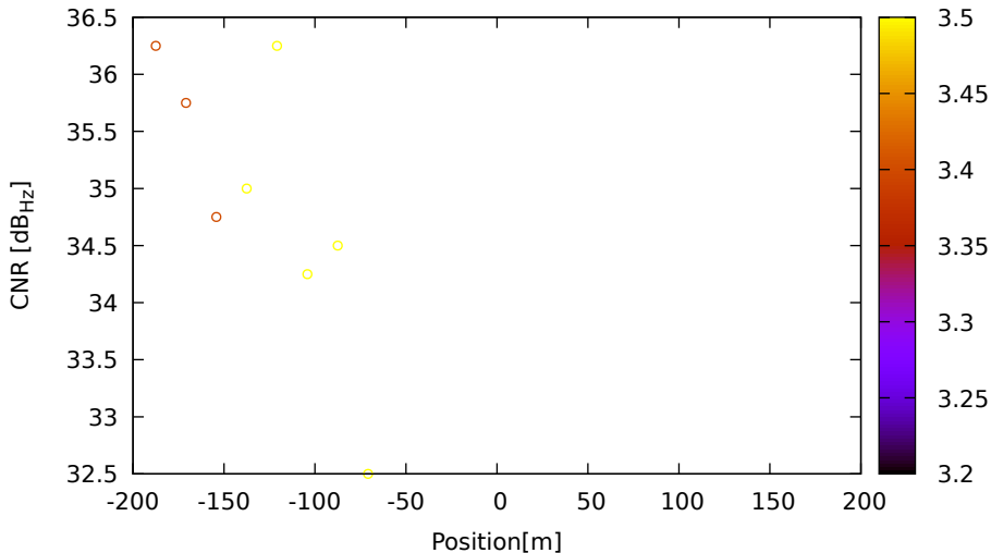
CNR vs position for R17 (G1) on LeicaGS18 - DOY 262 jam. 2
