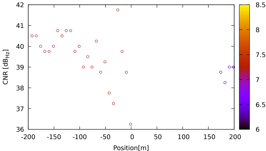
CNR vs position for R17 (G1) on LeicaGS18 - DOY 262 jam. 3
